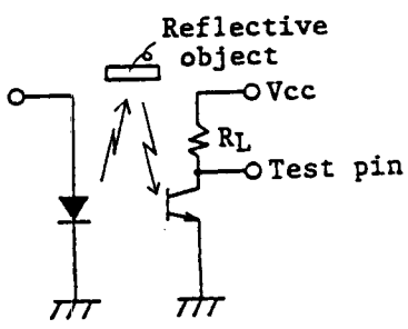
(Test circuit for response time)
