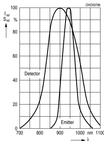
Relative Spectral Emission of Emitter (GaAs) and Detector (Si) I_{rel} = f(\lambda) and S_{rel} = f(\lambda)
