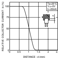
Fig.4 Relative output current vs. distance (II)
