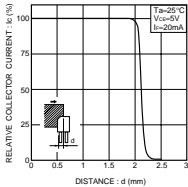
Fig.1 Relative output current vs. distance (I)
