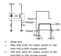
Fig.11 Response time measurement circuit
