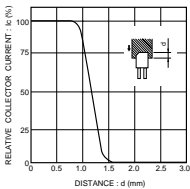
Fig.4 Relative output current vs. distance (1)
