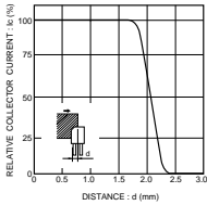
Fig.1 Relative output current vs. distance (1)
