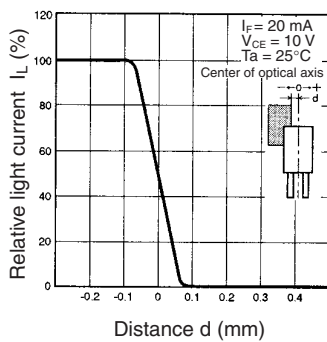
Sensing Position Characteristics (EE-SV3-C(S))
