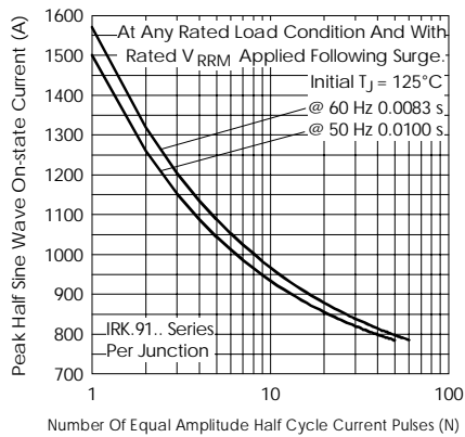
Fig. 13 - Maximum Non-Repetitive Surge Current
