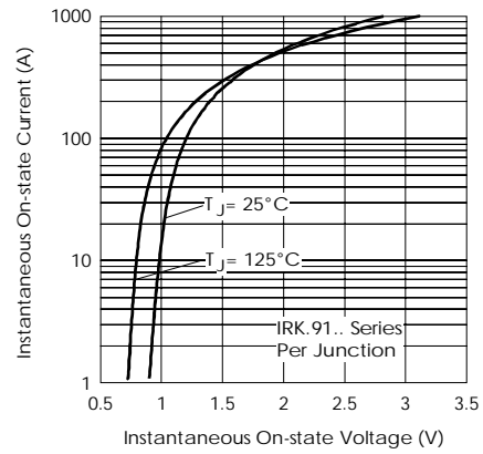
Fig. 18 - On-state Voltage Drop Characteristics
