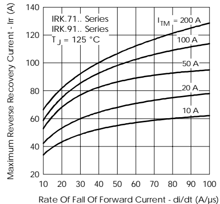
Fig. 20 - Recovery Current Characteristics
