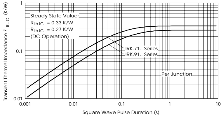
Fig. 21 - Thermal Impedance Z_{thJC} Characteristics
