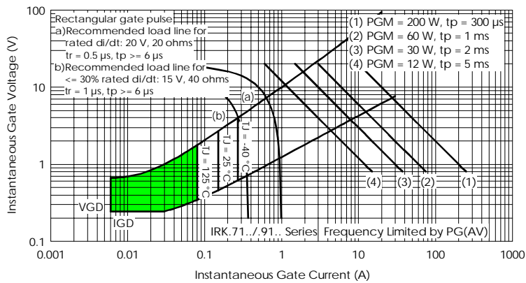
Fig. 22 - Gate Characteristics
