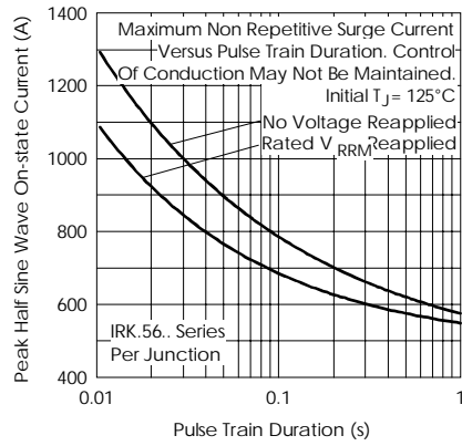
Fig. 14 - Maximum Non-Repetitive Surge Current
