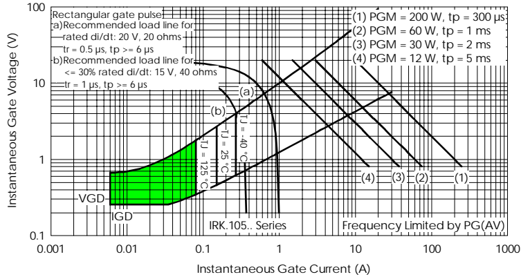
Fig. 14- Gate Characteristics
