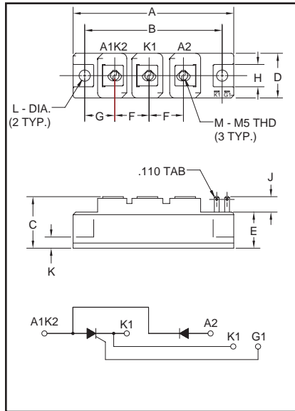
CM420855 SCR/Diode POW-R-BLOK™ Modules 55 Amperes/800 Volts
