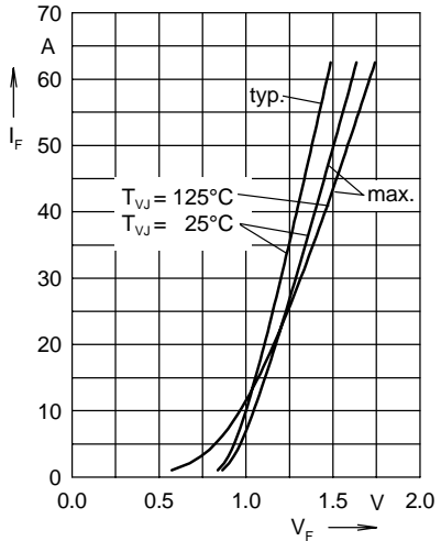
Fig. 3 Forward current versus voltage drop per diode
