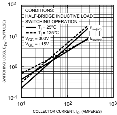
SWITCHING LOSS CHARACTERISTICS
