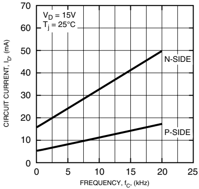
CIRCUIT CURRENT VS. FREQUENCY CHARACTERISTICS (TYPICAL)
