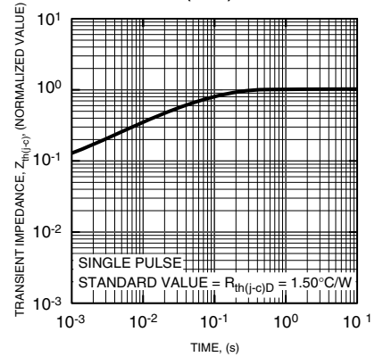
TRANSIENT THERMAL IMPEDANCE CHARACTERISTICS (FWD)
