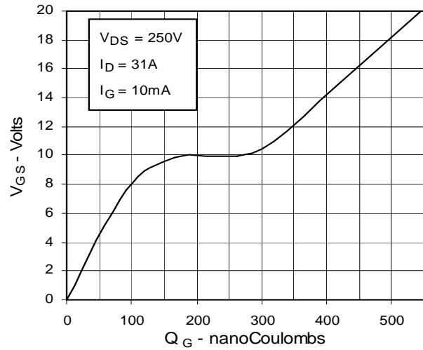
Fig. 10. Gate Charge
