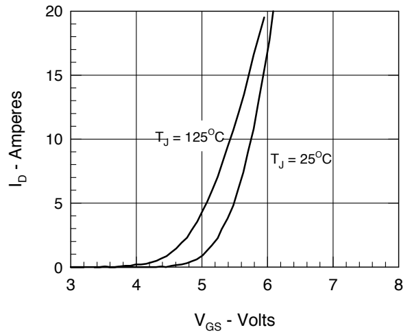
Figure 4. Admittance Curves
