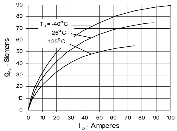
Fig. 8. Transconductance
