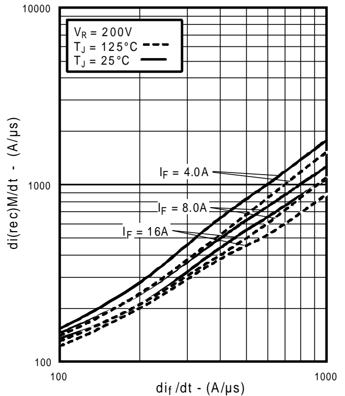
Fig. 17 - Typical di_{(rec)M}/dt vs. di_f/dt
