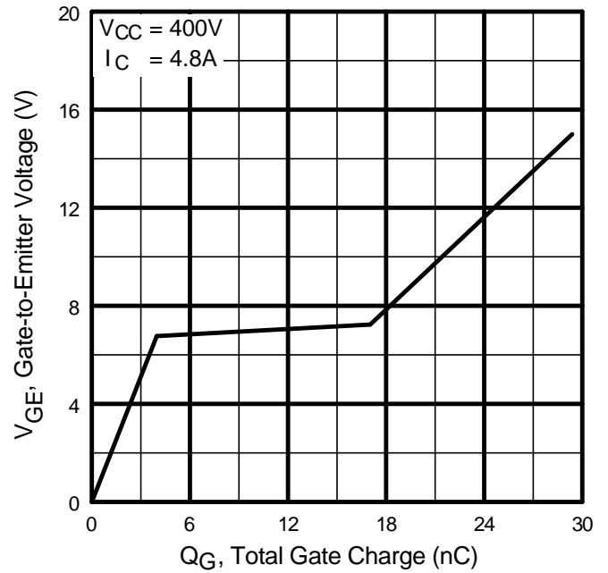
Fig. 8 - Typical Gate Charge vs. Gate-to-Emitter Voltage
