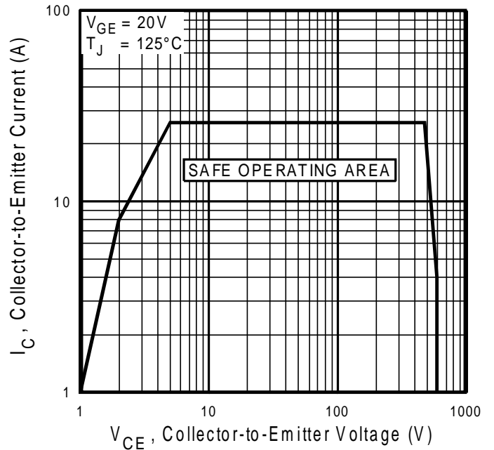
Fig. 12 - Turn-Off SOA
