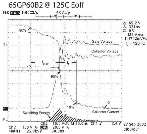
Figure 23, Turn-off Switching Waveforms and Definitions
