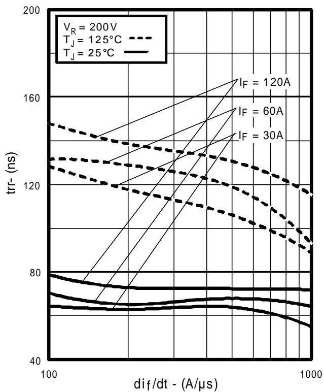
Fig. 5 - Typical Reverse Recovery vs. di_f/dt , (per Leg)
