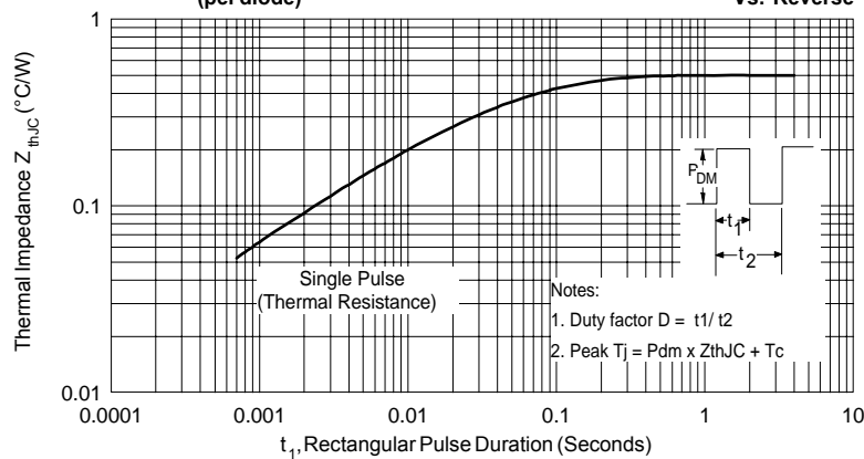
Fig. 4 - Max. Thermal Impedance Z_{thJC} Characteristics (per diode)
