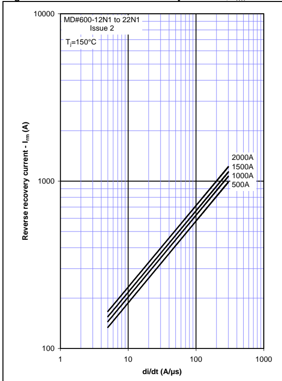
Figure 5 - Peak reverse recovery current, I_{rm}
