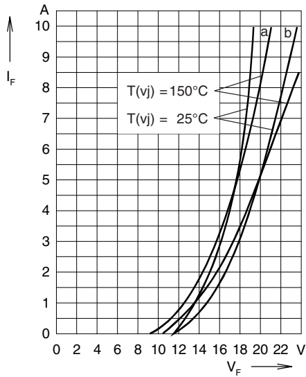
Fig. 1: Forward characteristics
