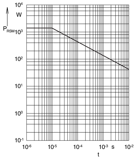
Fig. 3: Power loss
