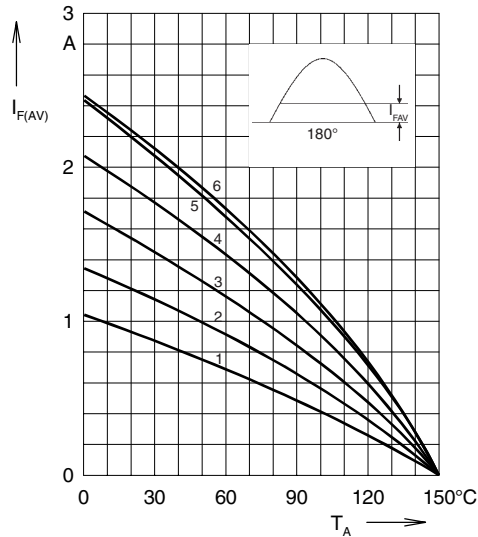
Fig. 4: Load diagram
