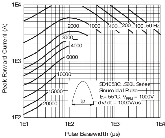
Fig. 35 - Frequency Characteristics
