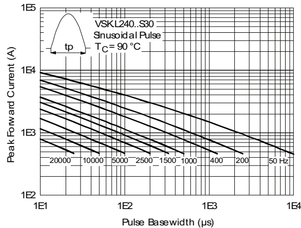
Fig. 25 - Frequency Characteristics
