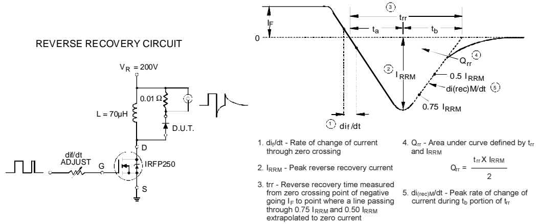
Fig. 10 - Reverse Recovery Waveform and Definitions
