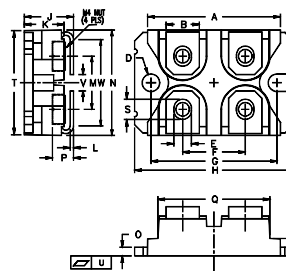
miniBLOC SOT-227 B M4 screws (4x) supplied
