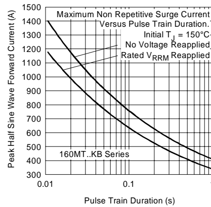
Fig. 10 - Maximum Non-Repetitive Surge Current
