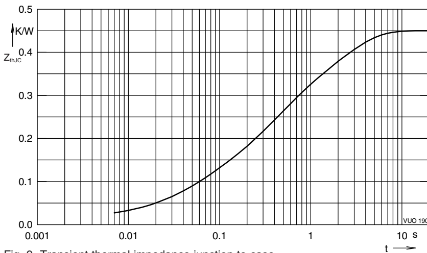
Fig. 9 Transient thermal impedance junction to case
