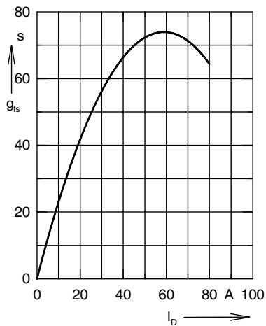
Fig. 9 Typ. transconductance, g_{is} = f(I_D) (MOSFET)
