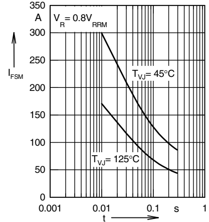
Fig. 1 Non-repetitive peak surge current (Rectifier Diodes)
