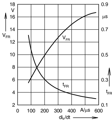
Fig. 15 Peak forward voltage versus -di_F/dt (Boost Diode)
