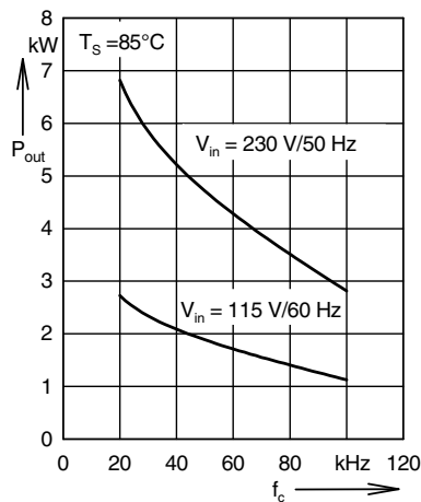
Fig. 16 Output power versus carrier frequency (Module)
