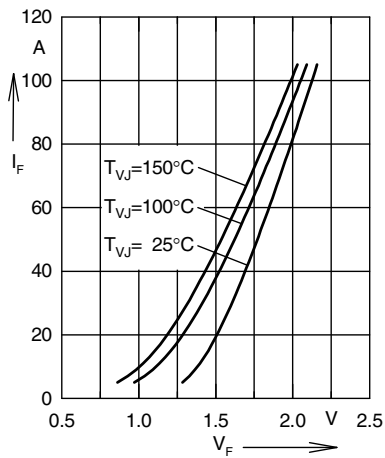
Fig. 10 Forward current versus voltage drop (Boost Diode)
