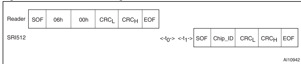
Figure 25. Initiate frame exchange between reader and SRI512
