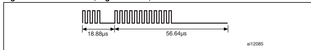
Figure 30. End of frame, high data rate, one subcarriers x2
