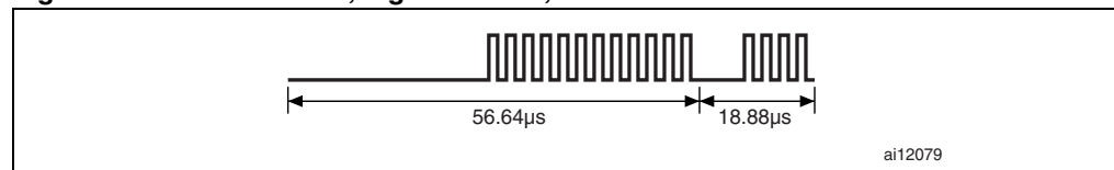
Figure 24. Start of frame, high data rate, one subcarrier x2
