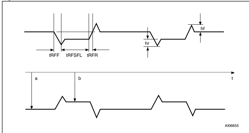
Figure 3. 10% modulation waveform
