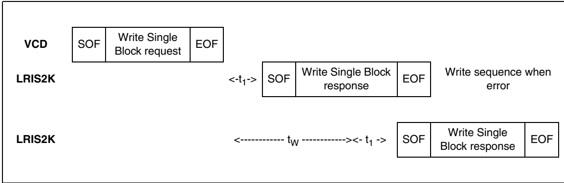
Figure 42. Write Single Block frame exchange between VCD and LRIS2K
