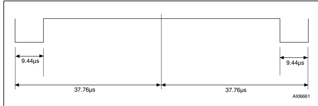
Figure 8. SOF to select 1 out of 256 data coding mode
