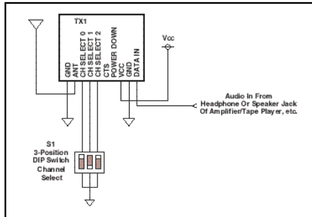
Figure 20: Typical Application: Voice Transmitter
