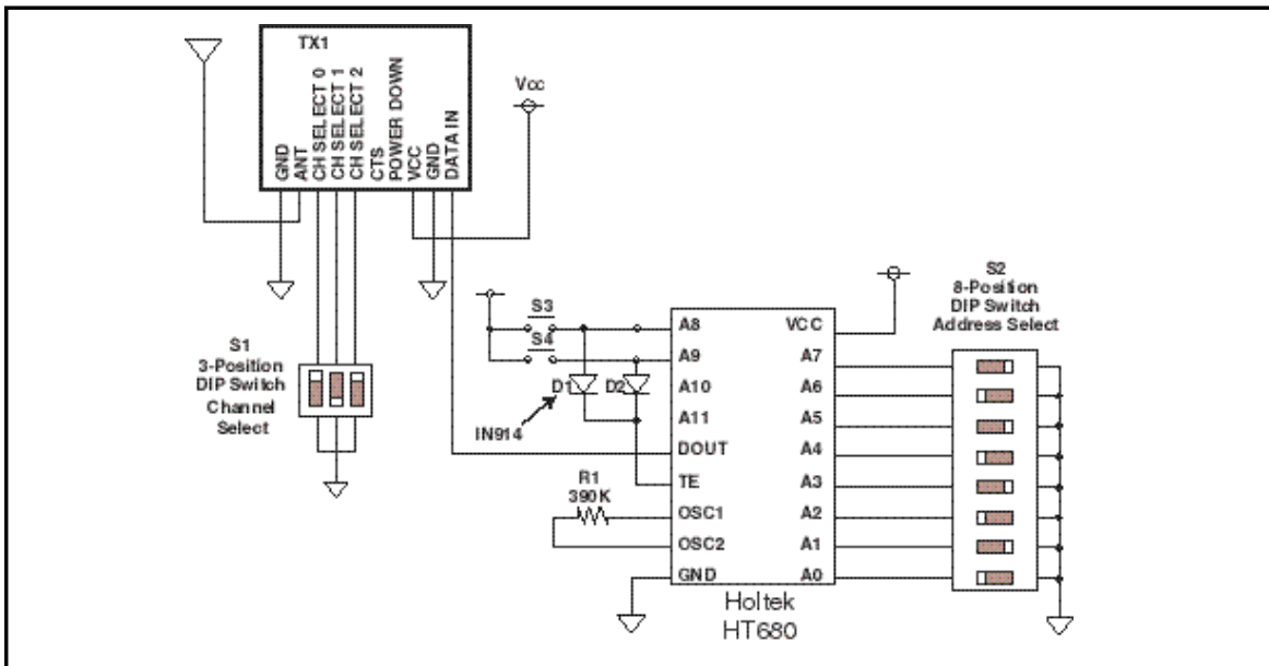
Figure 19: Typical Application: Remote-Control Transmitter
