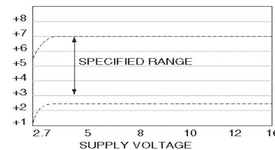
Figure 9: Output Power vs. Supply Voltage
