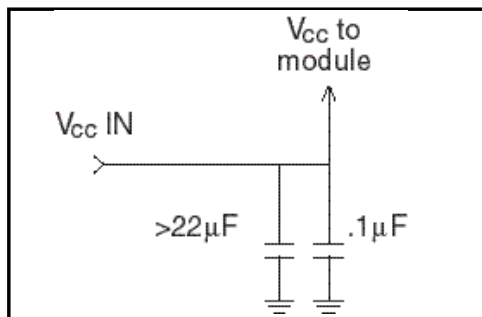
Figure 15: Suggested supply filter
