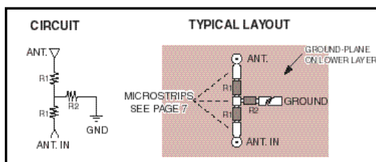
Figure 13A: Attenuation pad layout
