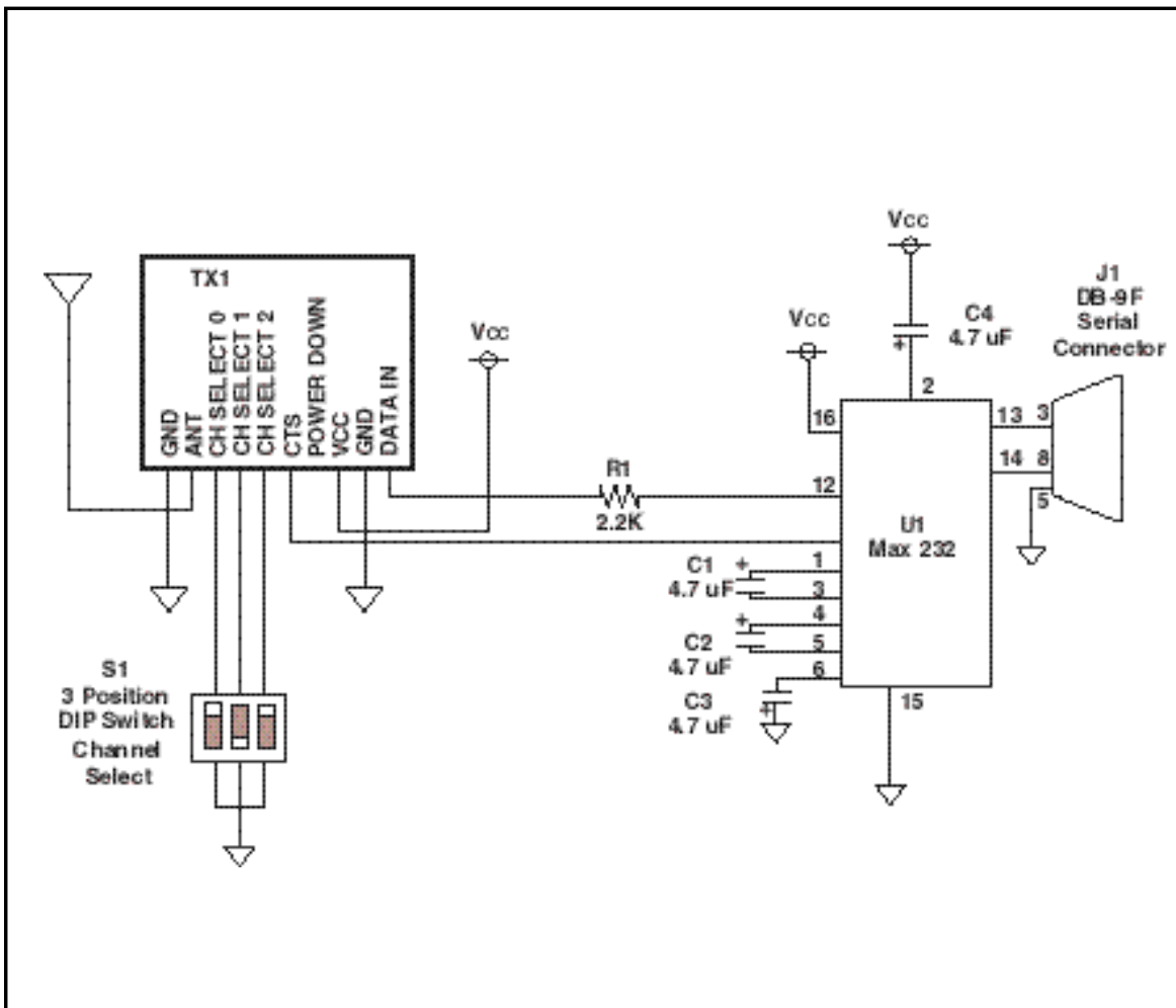
Figure 18: Typical Application: RS-232 Interface
