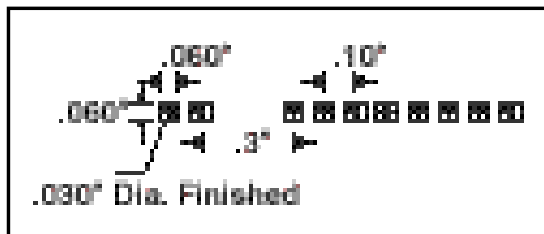
Figure 13: HP Series-II transmitter footprint
