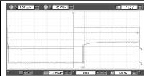
Figure 4: Power-On Timing
