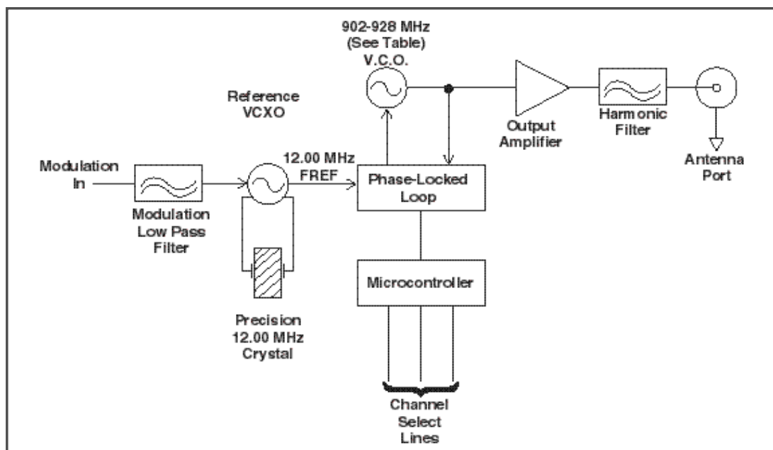
Figure 12: HP Series-II transmitter block diagram
