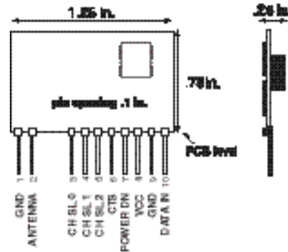
Figure 1: Physical Dimensions
