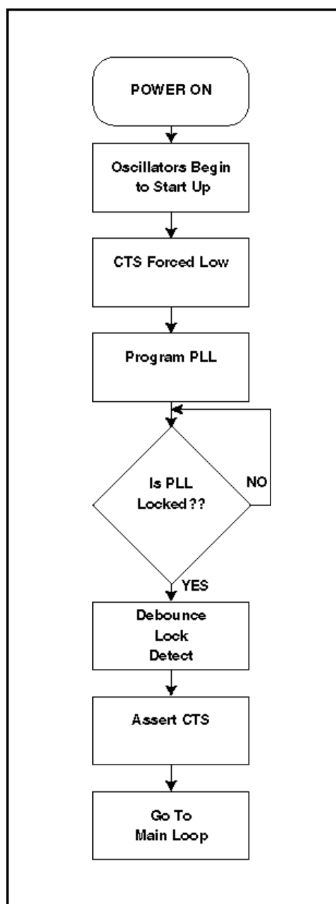
Figure 16: Start-up sequence
