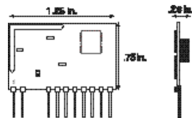
Figure 10: Physical package
