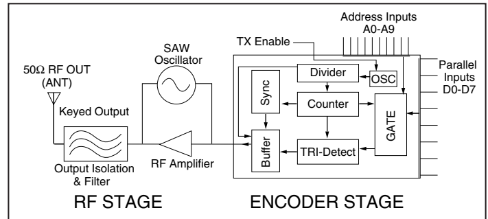
Figure 7: KH Series Transmitter Block Diagram
