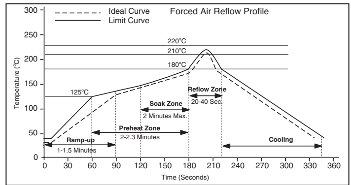
Figure 16: Maximum Reflow Profile
