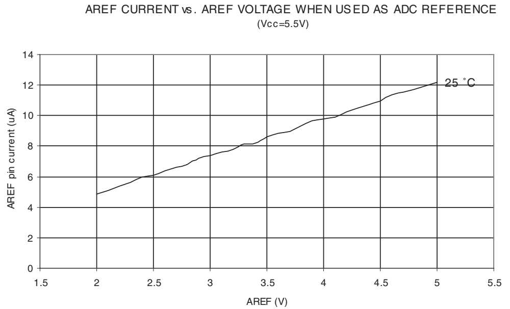
Figure 30-37. AREF External Reference Current vs. V_{CC}
