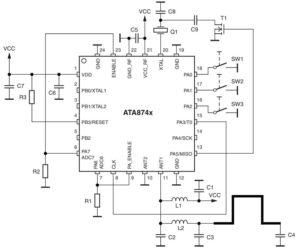
Figure 8-3. Typical FSK Application ATA8741
