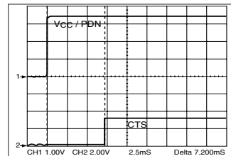
Figure 3: Power-Up to CTS
