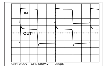
Figure 6: Square Wave Modulation Linearity
