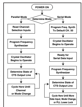
Figure 10: Start-up Sequence
