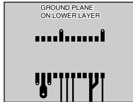
Figure 16: Suggested PCB Layout
