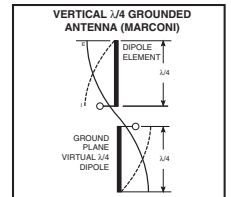
Figure 24: Dipole Antenna
