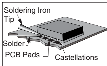
Figure 19: Soldering Technique
