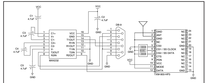
Figure 14: HP3 Transmitter and MAX232 IC
