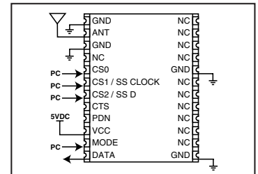
Figure 2: Test / Basic Application Circuit
