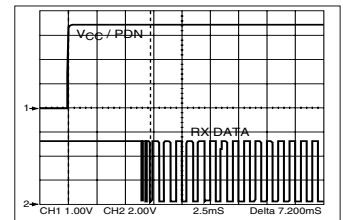
Figure 4: TX Power-up to Valid RX Data
