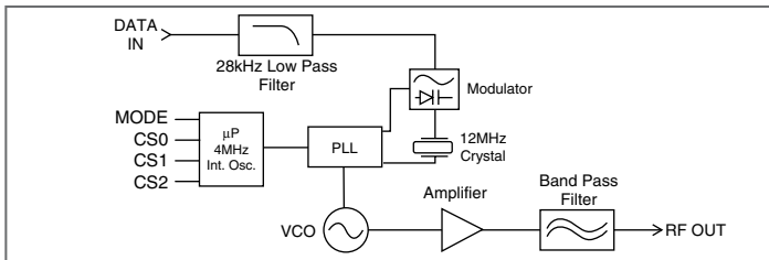
Figure 9: HP-3 Series Transmitter Block Diagram
