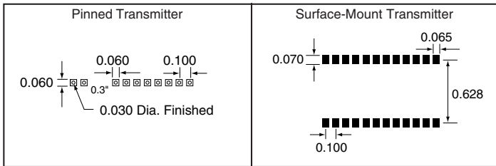
Figure 18: Recommended PCB Layout
