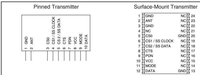
Figure 7: HP3 Series Receiver Pinout
