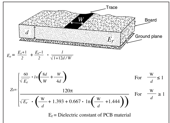
Figure 17: Microstrip Formulas
