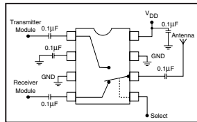
Figure 22: Typical Antenna Switch
