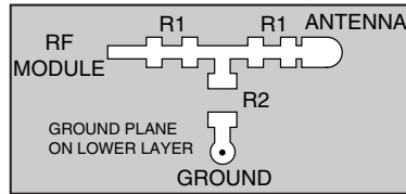
Figure 12: T-Pad Attenuator Example Layout
