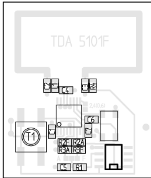
Figure 4-5 Top Side of TDA 5101-Application Board
