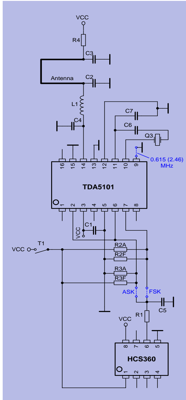
Figure 4-4 Application board schematic
