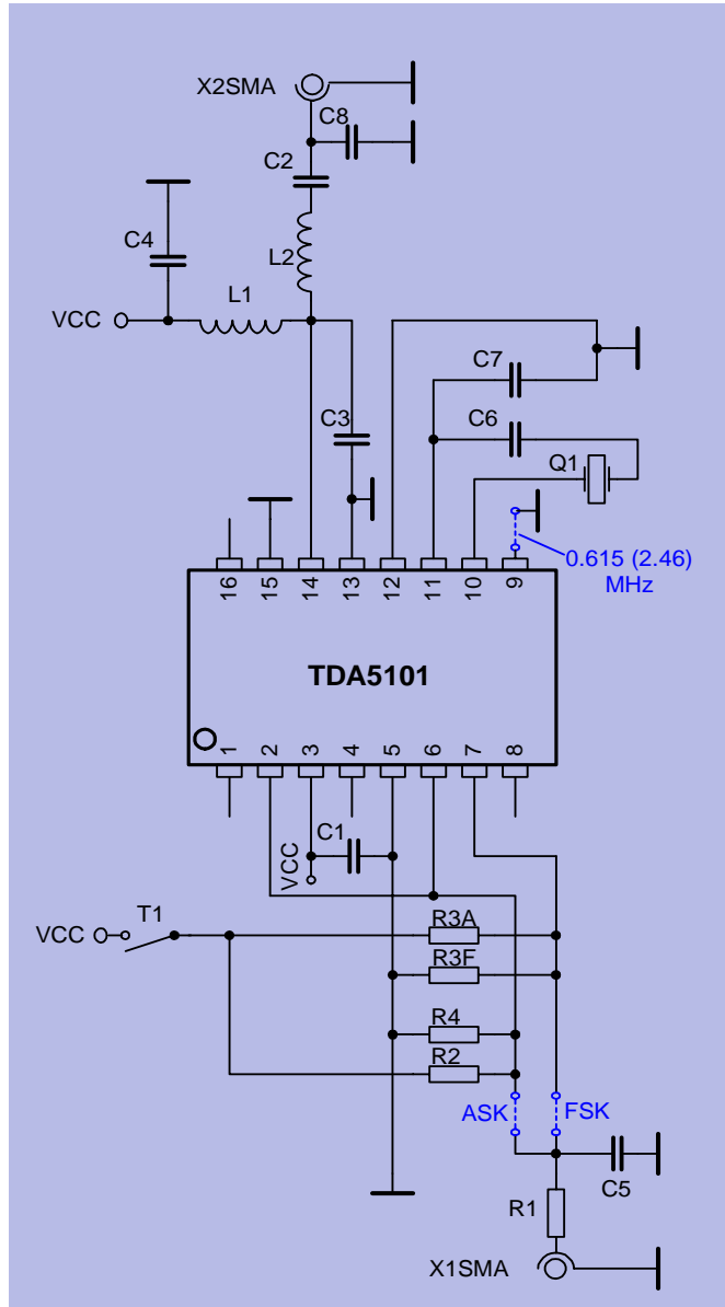
Figure 4-1 50 Ω-Output testboard schematic
