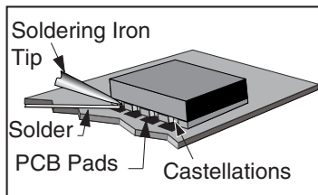
Figure 19: Soldering Technique
