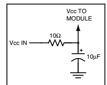
Figure 11: Supply Filter
