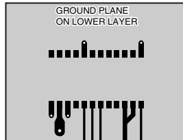
Figure 16: Suggested PCB Layout
