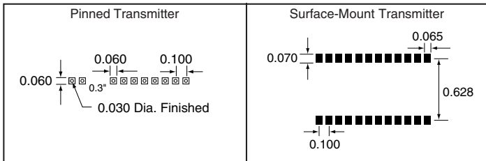
Figure 18: Recommended PCB Layout
