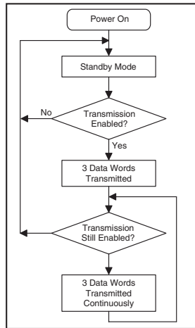
Figure 8: Encoder Flowchart
