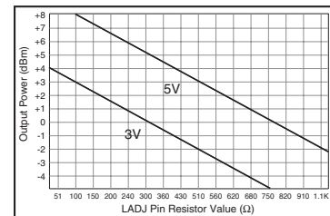
Figure 5: Output Power vs. LADJ Resistor
