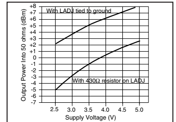
Figure 4: Output Power vs. Supply Voltage
