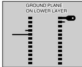
Figure 12: Suggested PCB Layout
