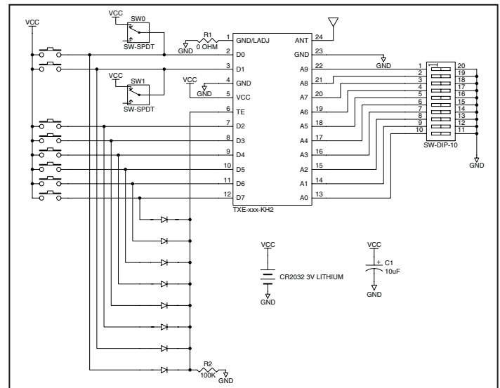
Figure 11: Basic Remote Control Transmitter
