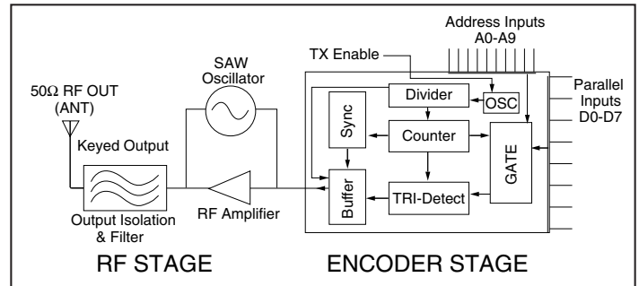
Figure 7: KH2 Series Transmitter Block Diagram
