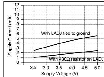
Figure 3: Supply Current vs. Supply Voltage
