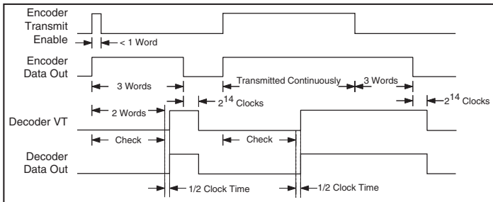
Figure 9: Encoder / Decoder Timing Diagram
