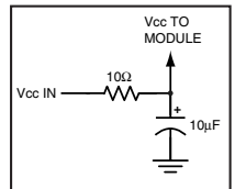
Figure 10: Supply Filter
