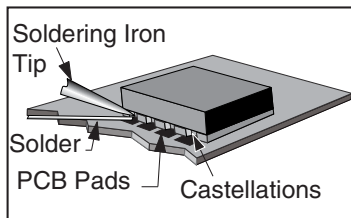
Figure 14: Soldering Technique
