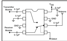
Figure 17: Typical Antenna Switch
