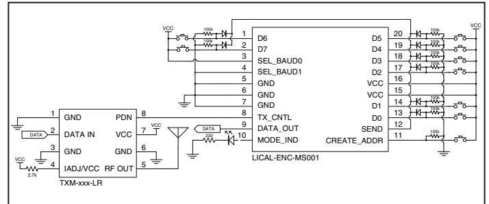
Figure 8: LR Transmitter and MS Encoder
