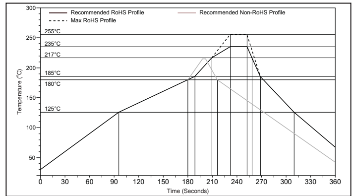
Figure 15: Maximum Reflow Profile
