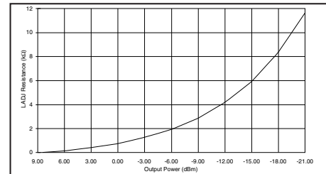
Figure 4: Output Power vs. LADJ Resistance
