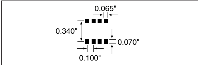
Figure 13: Recommended PCB Layout
