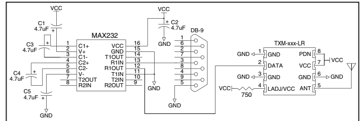
Figure 9: LR Transmitter and MAX232 IC
