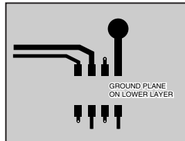
Figure 11: Suggested PCB Layout
