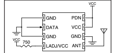
Figure 2: Test / Basic Application Circuit
