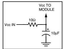
Figure 7: Supply Filter
