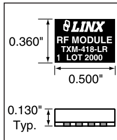
Figure 1: Package Dimensions
