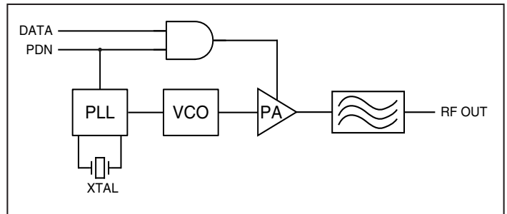
Figure 6: LR Series Transmitter Block Diagram
