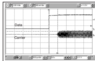
Figure 5: Typical Oscillator Turn-On Time
