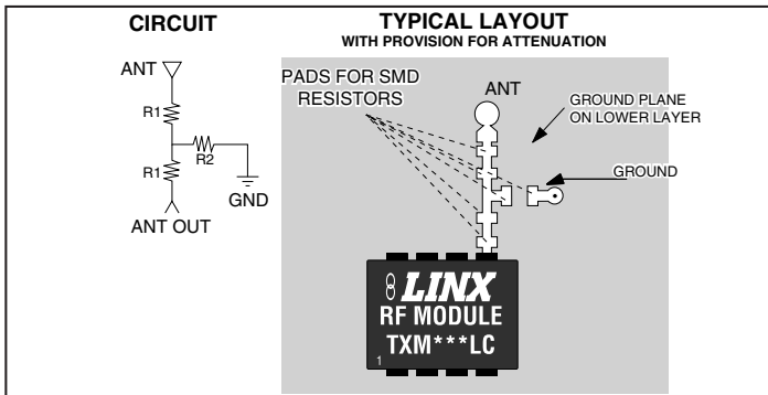
Figure 10: A T-Pad Attenuator Layout Example
