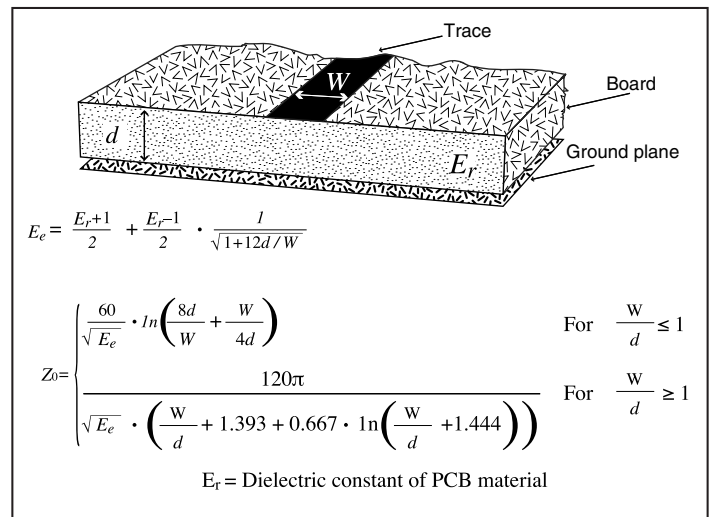
Figure 12: Microstrip Formulas
