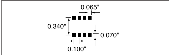
Figure 15: Recommended PCB Layout
