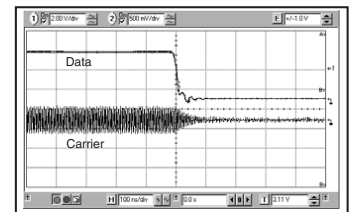
Figure 6: Typical Oscillator Turn-Off Time
