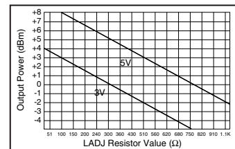
Figure 7: Output Power vs. LADJ Resistor
