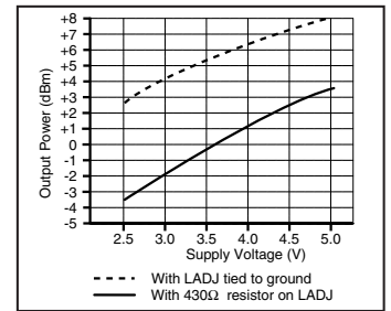
Figure 4: Output Power vs. Supply Voltage
