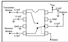
Figure 19: Typical Antenna Switch
