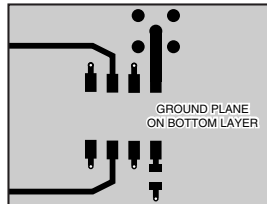
Figure 13: Suggested PCB Layout
