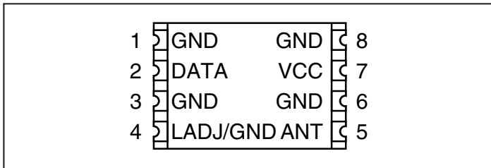
Figure 8: LC Series Transmitter Pinout (Top View)
