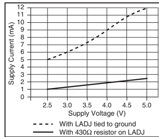
Figure 3: Current vs. Supply Voltage
