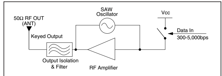
Figure 9: LC Series Transmitter Block Diagram
