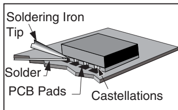
Figure 16: Soldering Technique
