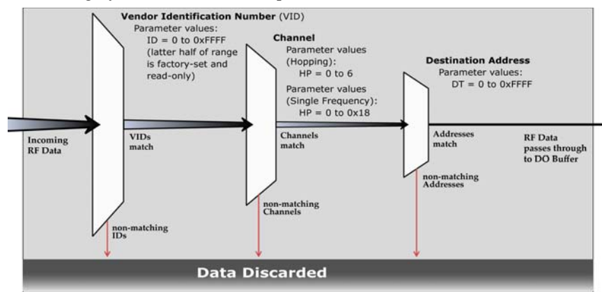
Figure 5-01. Addressing layers contained in the RF packet header
