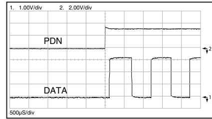
Figure 10: RX Turn-On Time from PDN
