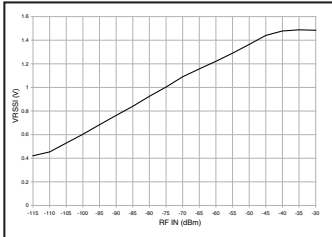
Figure 5: RSSI Curve
