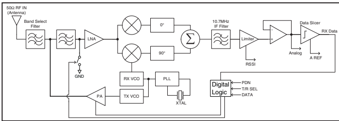
Figure 17: LT Series Transceiver Block Diagram
