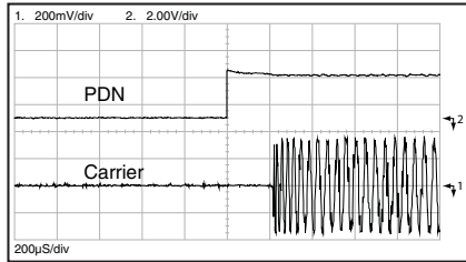
Figure 13: TX Turn-On Time from PDN
