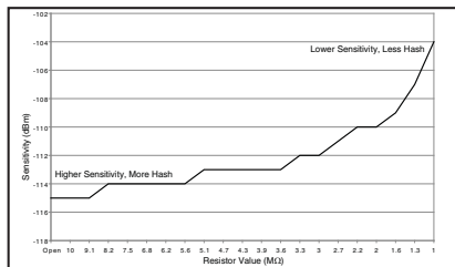
Figure 20: Sensitivity Degradation vs. Squelch Resistor
