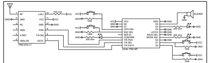
Figure 21: LT Transceiver and MT Transcoder
