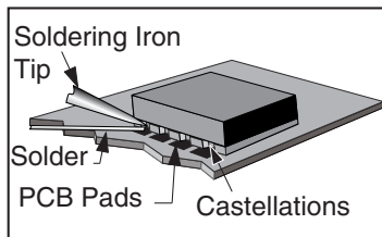
Figure 25: Soldering Technique
