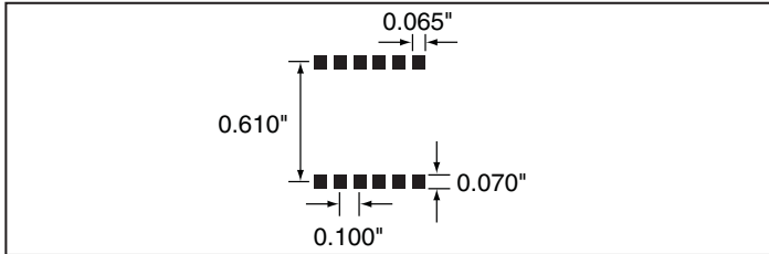
Figure 24: Recommended PCB Layout
