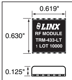
Figure 1: Package Dimensions
