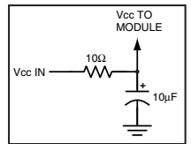
Figure 19: Supply Filter
