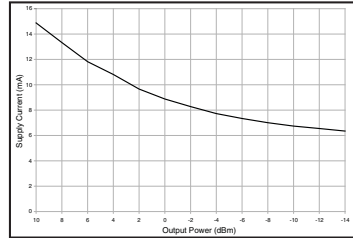
Figure 4: Output Power vs Current Consumption
