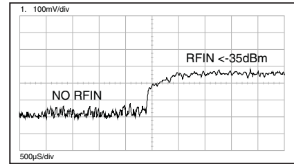
Figure 11: RSSI Response Time
