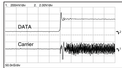
Figure 12: TX Modulation Delay
