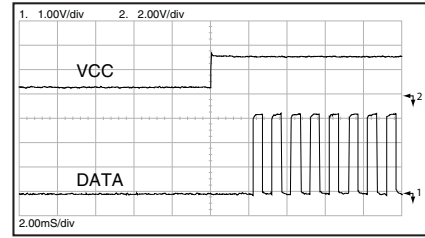
Figure 9: RX Turn-On Time from V_{CC}
