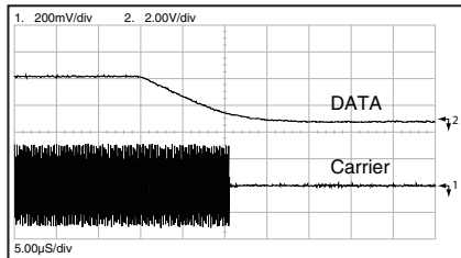
Figure 15: TX Turn-Off Time
