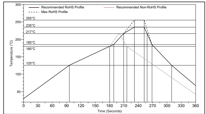
Figure 26: Maximum Reflow Profile
