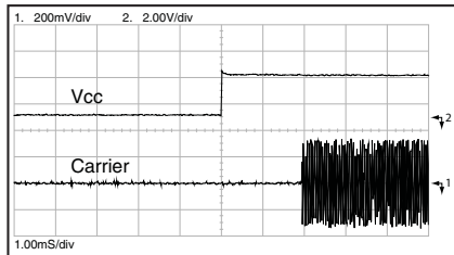
Figure 14: TX Turn-On Time from V CC
