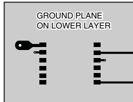
Figure 22: Suggested PCB Layout
