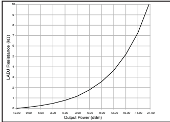
Figure 3: Output Power vs. LADJ Resistance
