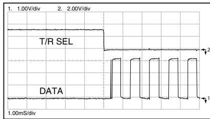
Figure 8: TX to RX Change Time
