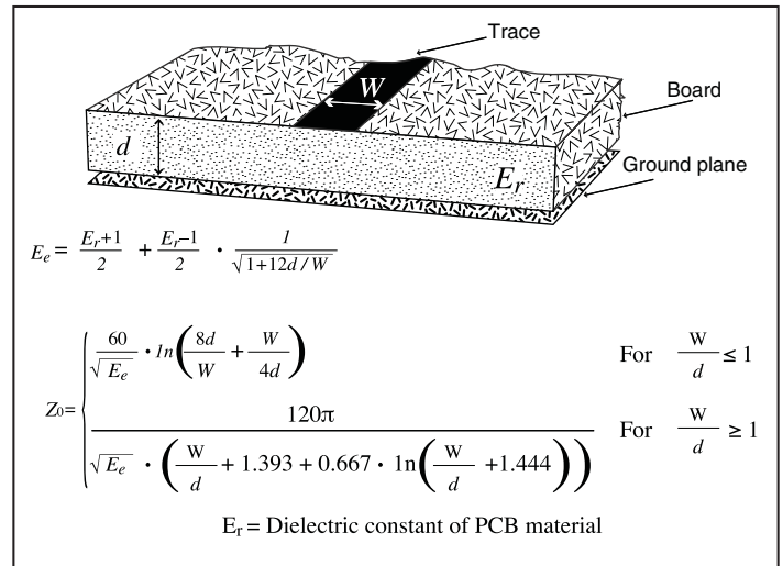
Figure 23: Microstrip Formulas
