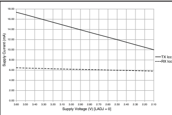
Figure 6: Current Consumption vs. Supply
