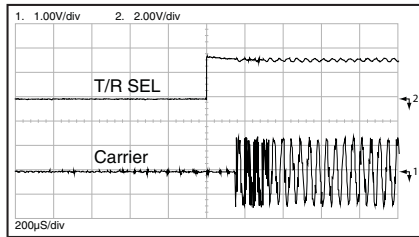
Figure 7: RX to TX Change Time
