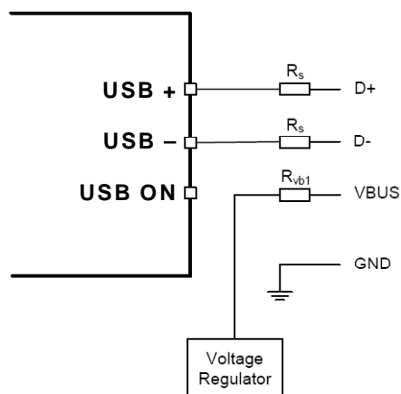
Connections to F2M03 for Bus-Powered Mode
