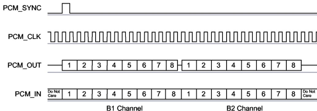
GCI Interface
