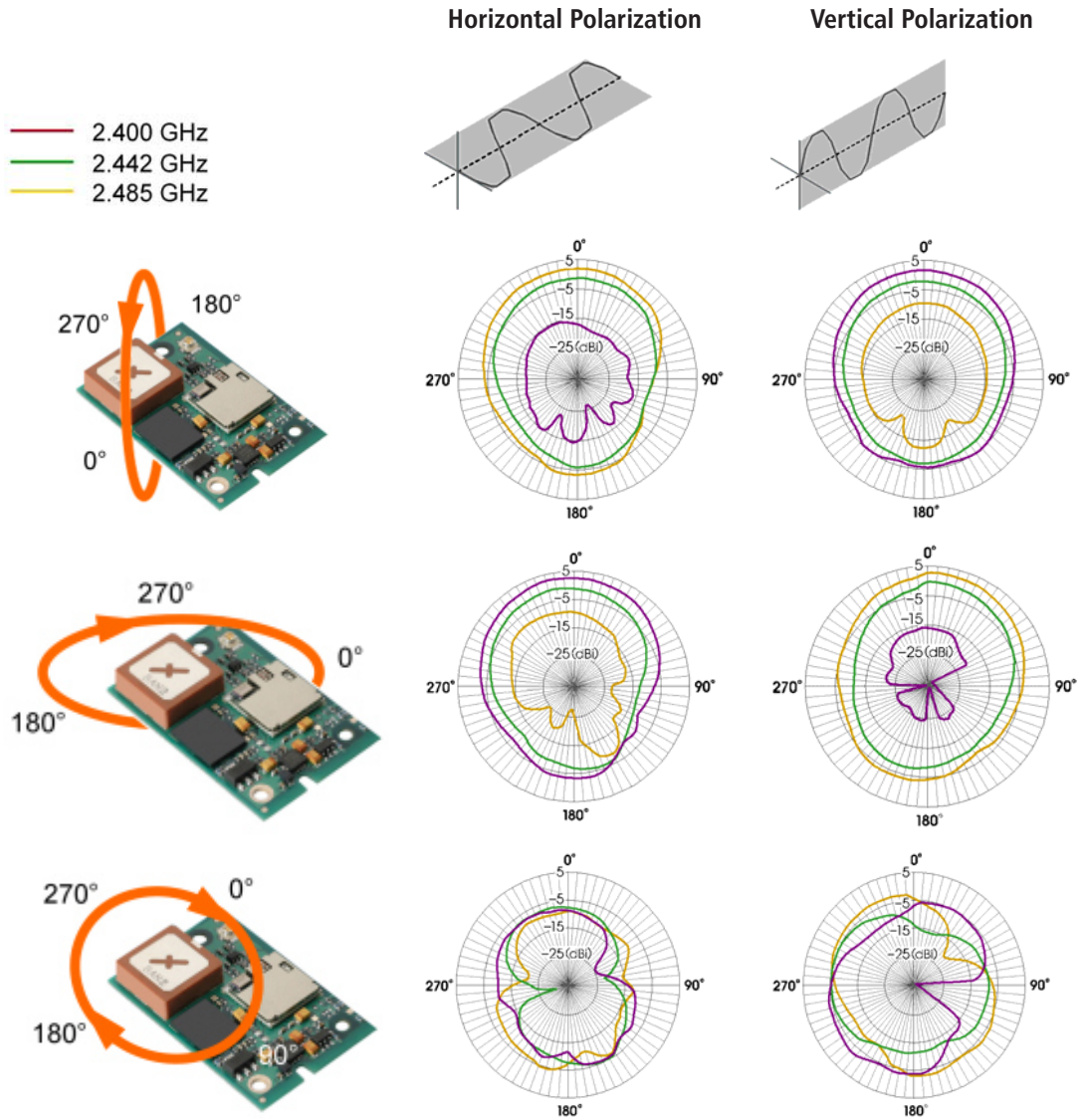
Typical Radiation Characteristics. Measured at 2.5 meters from a standard dipole.
