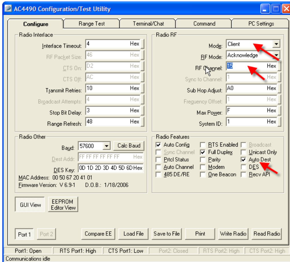
Figure 21: Client Settings
