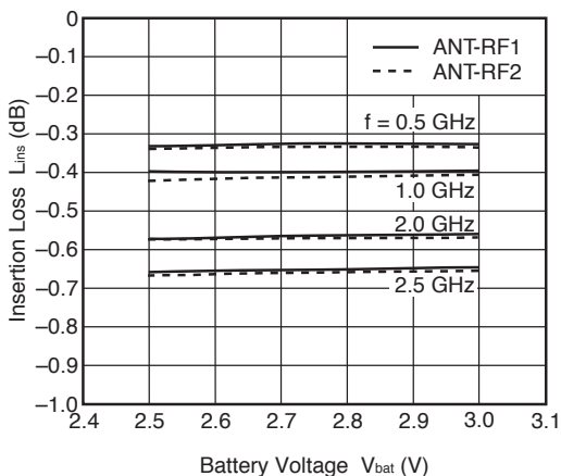
INSERTION LOSS vs. BATTERY VOLTAGE
