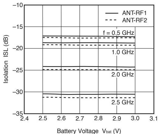
ISOLATION vs. BATTERY VOLTAGE
