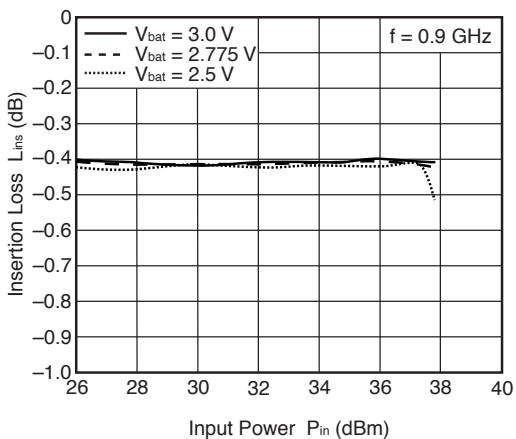
INSERTION LOSS vs. INPUT POWER
