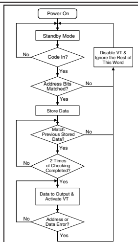
Figure 9: Decoder Flowchart
