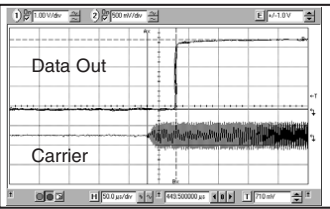
Figure 5: RF In vs. Receiver Response Time
