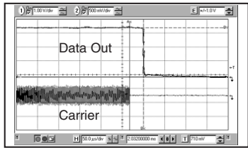
Figure 6: Receiver Turn-Off Time
