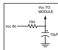
Figure 11: Supply Filter
