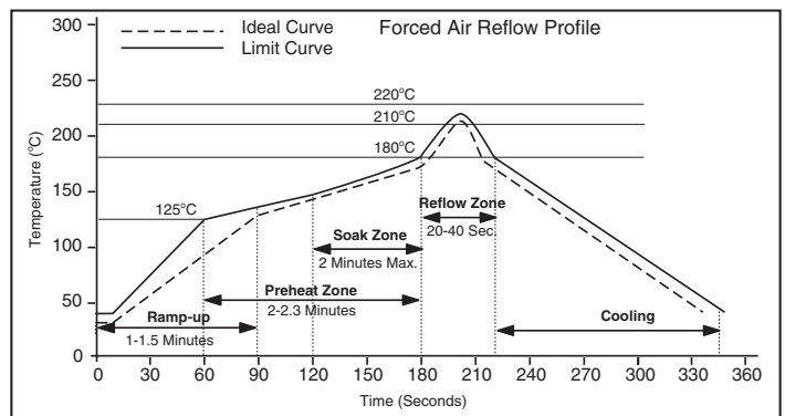
Figure 19: Maximum Reflow Profile
