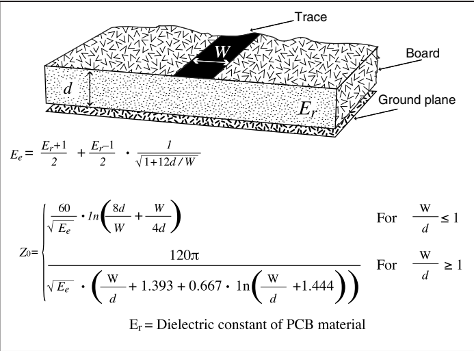
Figure 16: Microstrip Formulas
