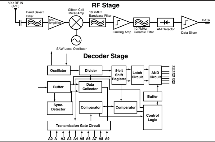
Figure 8: KH Series Receiver Block Diagram
