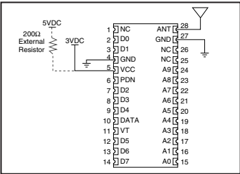
Figure 2: Test / Basic Application Circuit
