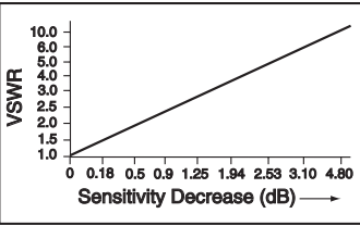
Figure 3: Sensitivity vs. VSWR
