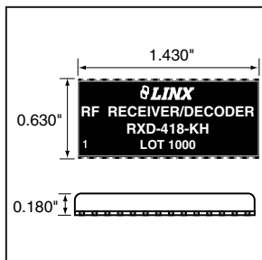
Figure 1: Package Dimensions
