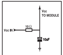
Figure 15: Supply Filter
