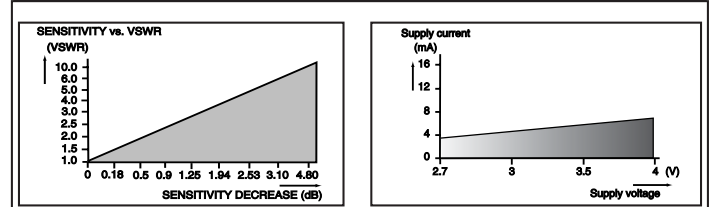
Figure 3: Sensitivity vs. VSWR
