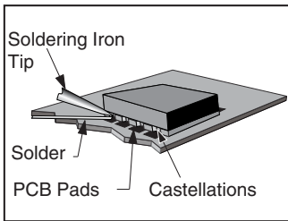
Figure 11: LC-S Soldering Technique
