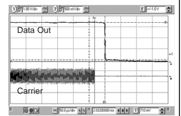
Figure 6: Typical Receiver Turn-Off Time
