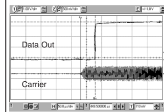
Figure 5: RF in vs. Receiver Response Time
