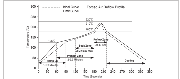
Figure 12: Required Reflow Profile
