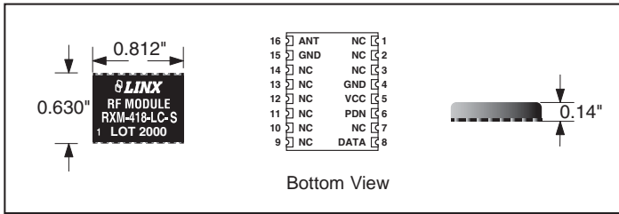
Figure 2: LC-S Series Receiver Package Dimensions
