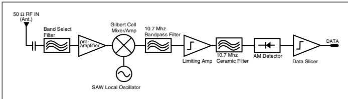
Figure 13: LC Series Receiver Block Diagram
