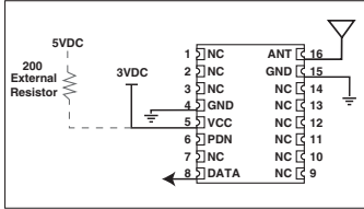
Figure 1: Test/Basic Application Circuit
