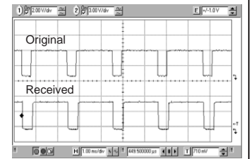
Figure 8: Original vs. Received Data 4,800bps 80% Duty Cycle
