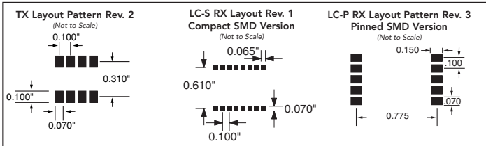
Figure 10: Recommended Pad Layout
