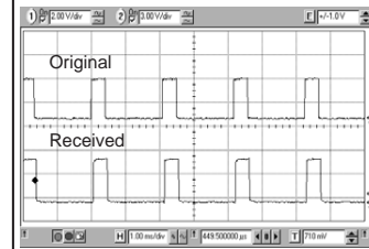
Figure 7: Original vs. Received Data 4,800bps 20% Duty Cycle
