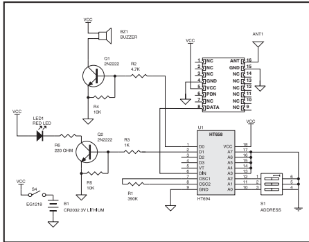
Figure 16: Basic Remote Control Receiver
