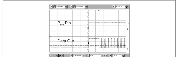
Figure 9: Power-On Settling Time (Time to Valid Data)
