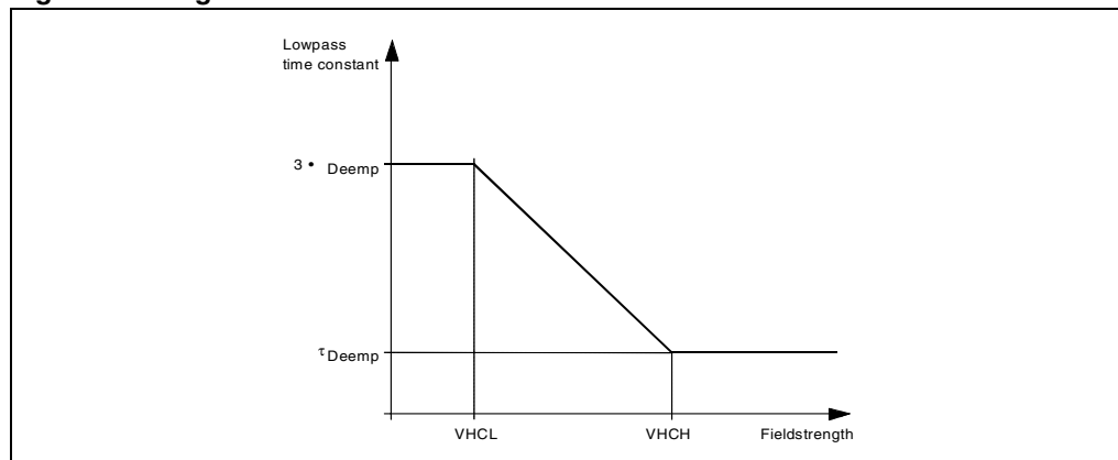
Figure 7. Highcut characteristics
