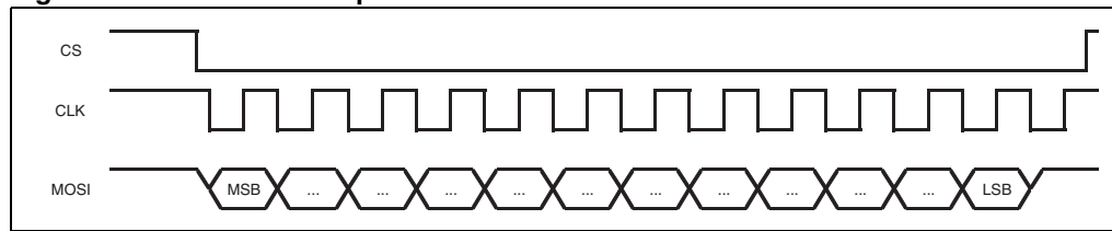
Figure 6. SPI "write" sequence
